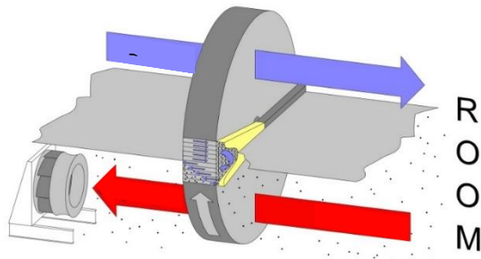
Figure 15. Purge sector
