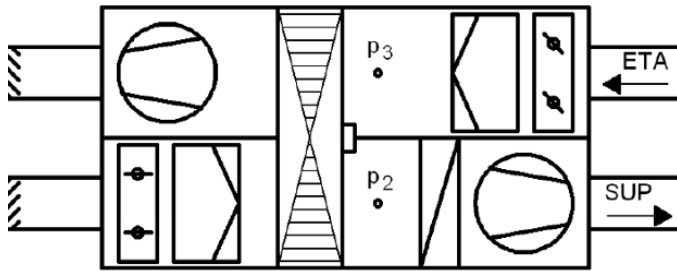
Figure 14. Throttling
