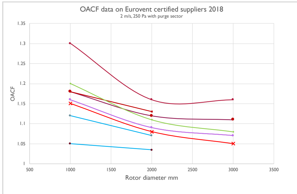
Figure 8. Typical OACF values from Eurovent certified suppliers
