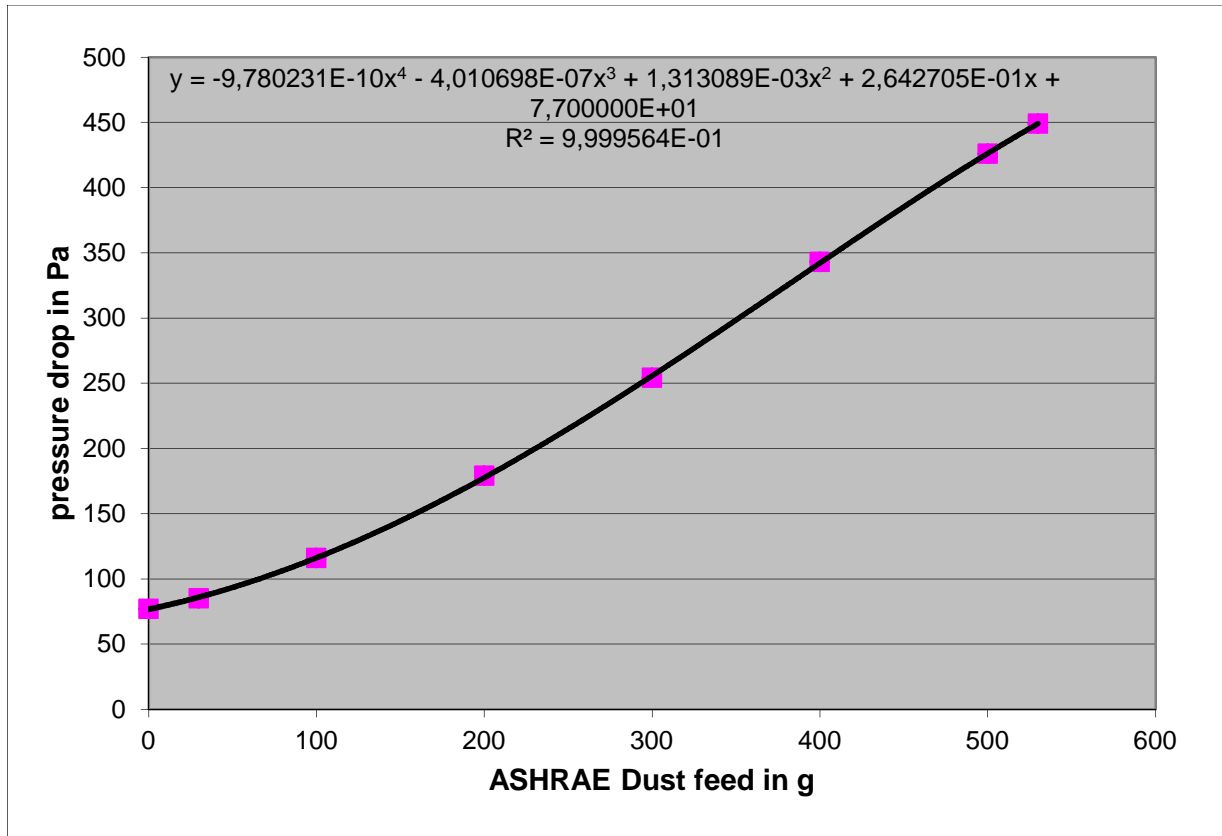
Figure 1: Pressure drop as a function of the dust loading as result of the EN 779 test at 0.944 m 3 /s. The function plotted on the top of the diagram shows the parameters a , b , c and d of Eq. (2) resulting from a curve fit of a polynomial of 4 th order to the test data and the related coefficient of determination R^2 .
