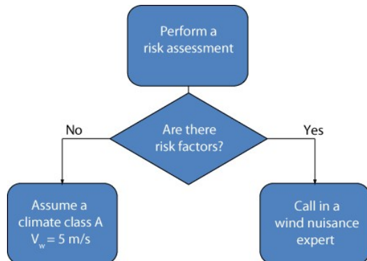
Figure 13: Working method assessment of wind nuisance risk
