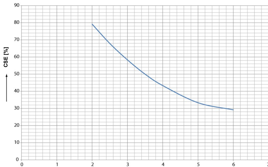
Figure 2: CSE in% as a function of the pressure difference over the air jet
