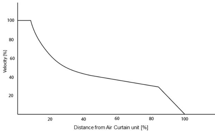
Figure 4: example of the air velocity of an installed air curtain unit
