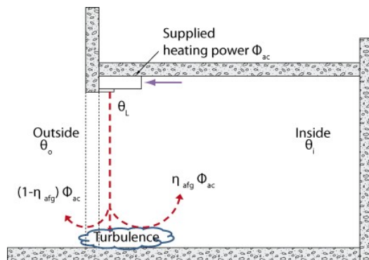
Figure 8: Supply performance of a heated air curtain
